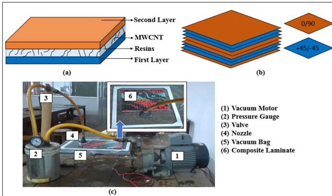
(a) Three phased composite, (b) Symmetrical laminate design and (c) Vacuum bagging set-up.
